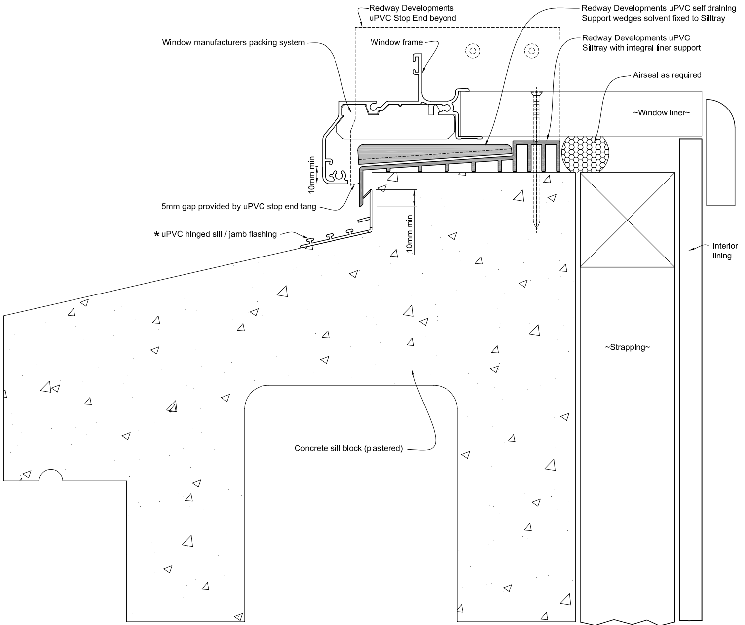
Section Through Sill
