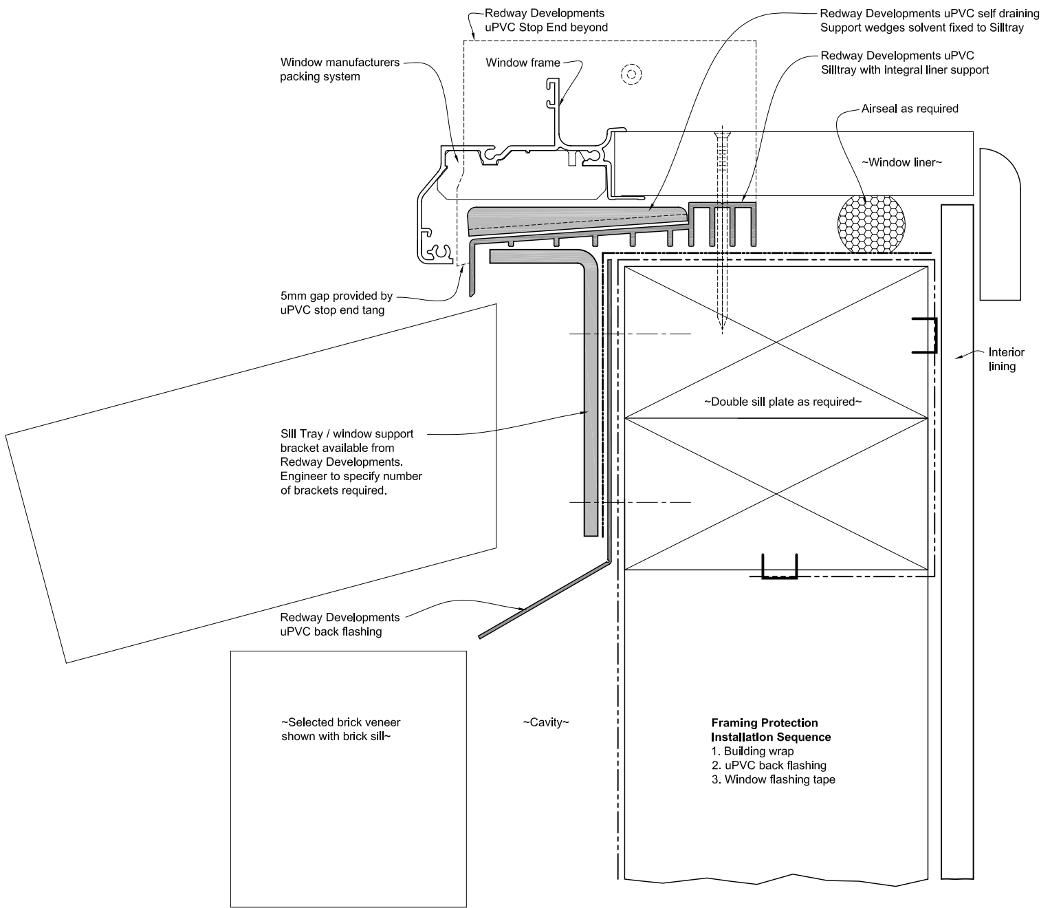
Section Through Sill
