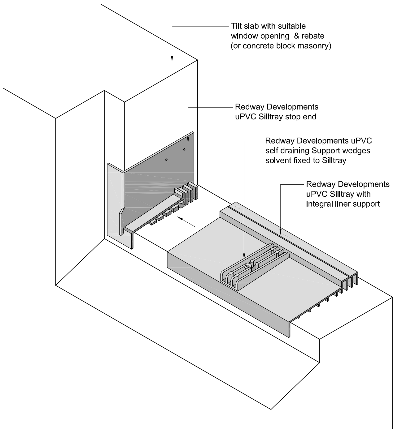
Typical Tilt Slab (Or Concrete Block) At Window Opening
