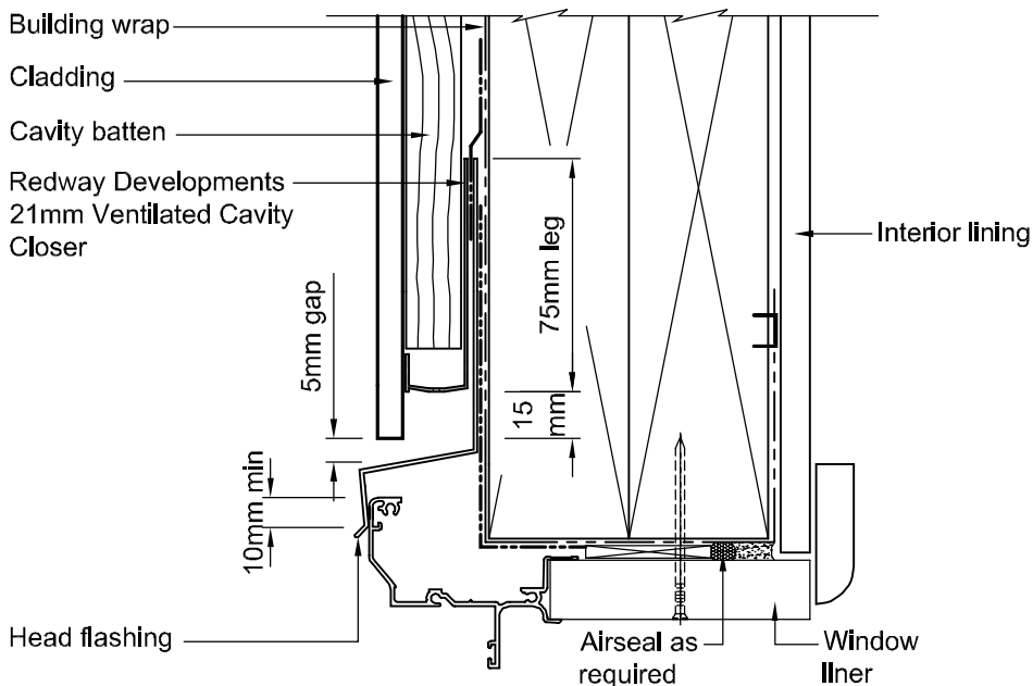
Window or Door Head
