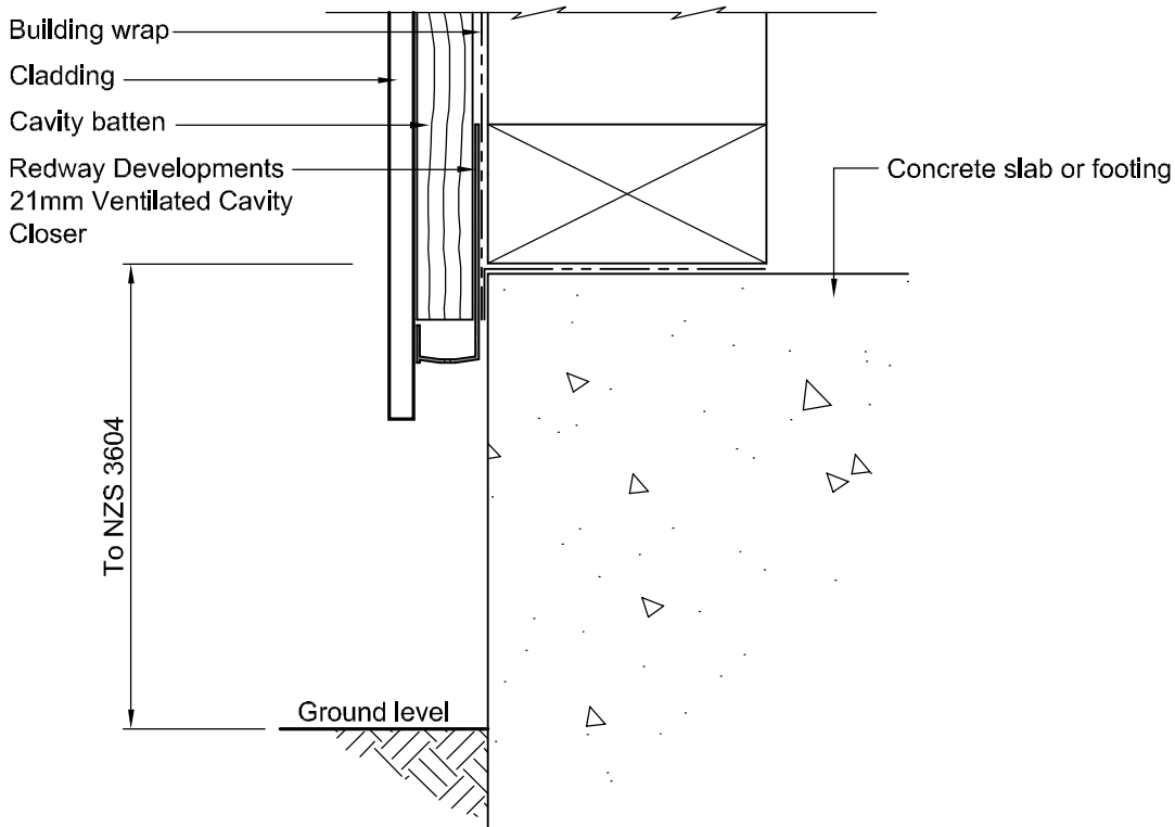
Wall to Concrete Slab
