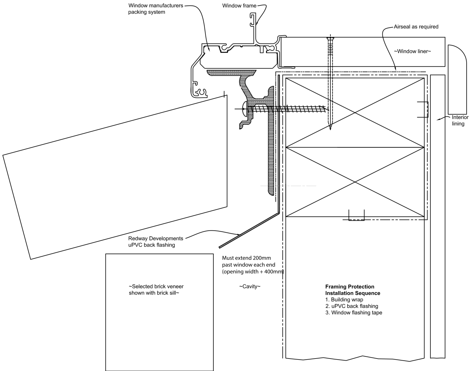
Section Through Sill
